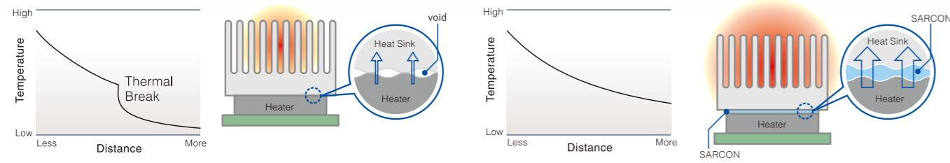
Thermal resistance of semiconductor mounted to substrate is appreciably increased at junction of porous surfaces.
